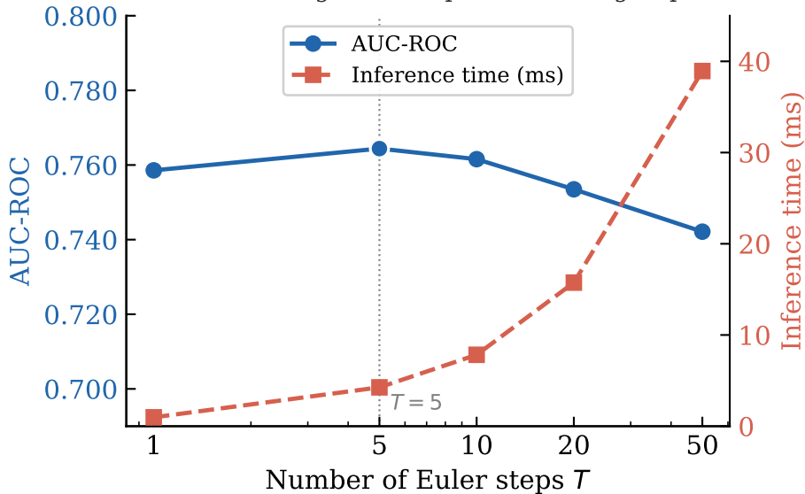
Effect of integration steps on 20Newsgroups
